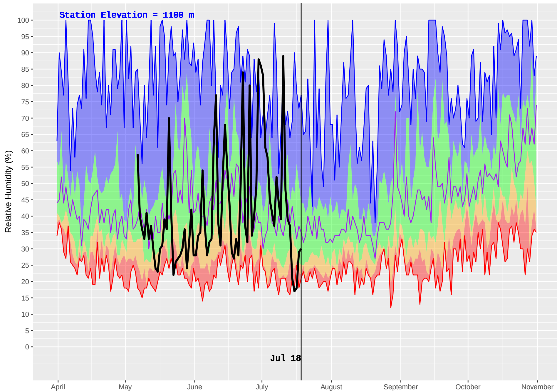
CHURN CREEK (832) : Historical (2003–2016) and Current (2018) Daily Relative Humidity
