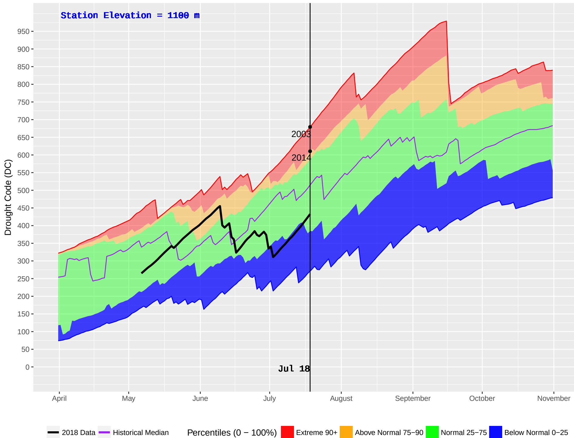
CHURN CREEK (832) : Historical (2003–2016) and Current (2018) Daily Drought Code (DC)
